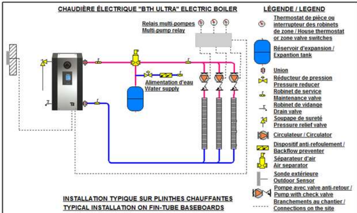
Figure 6 : Installation multi-pompes
