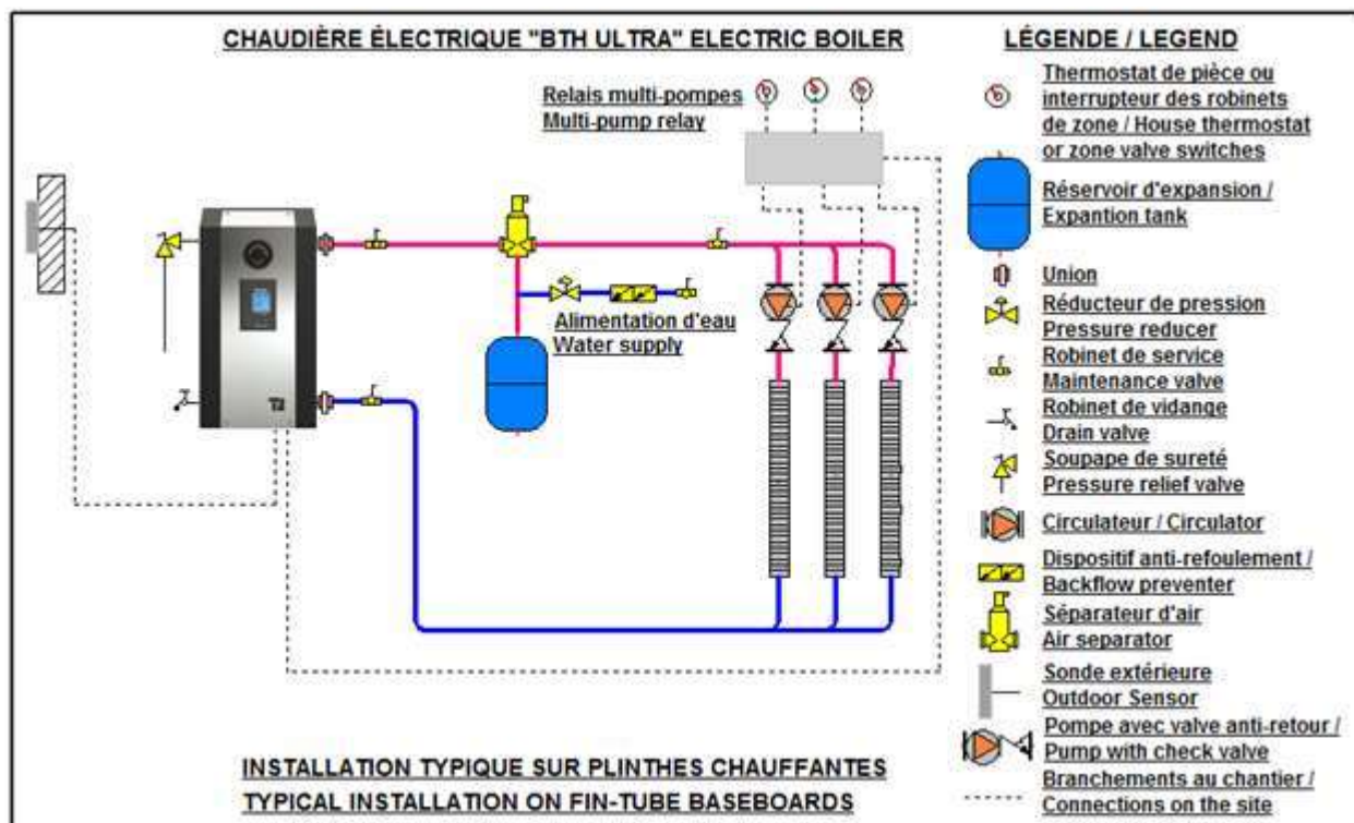
Figure 5 : Installation multi-pompes
