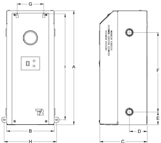
Figure 1 : Dimensions
