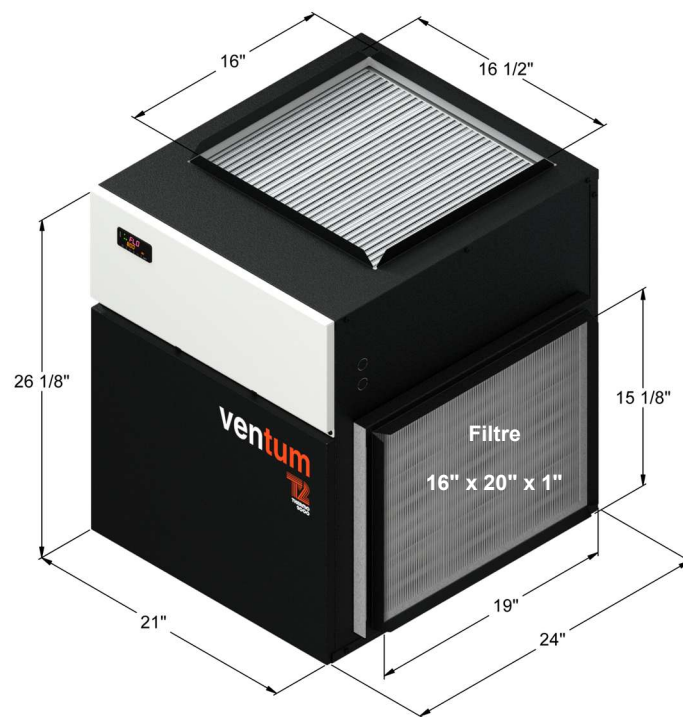
Figure 1 : Dimensions VenTum 40
