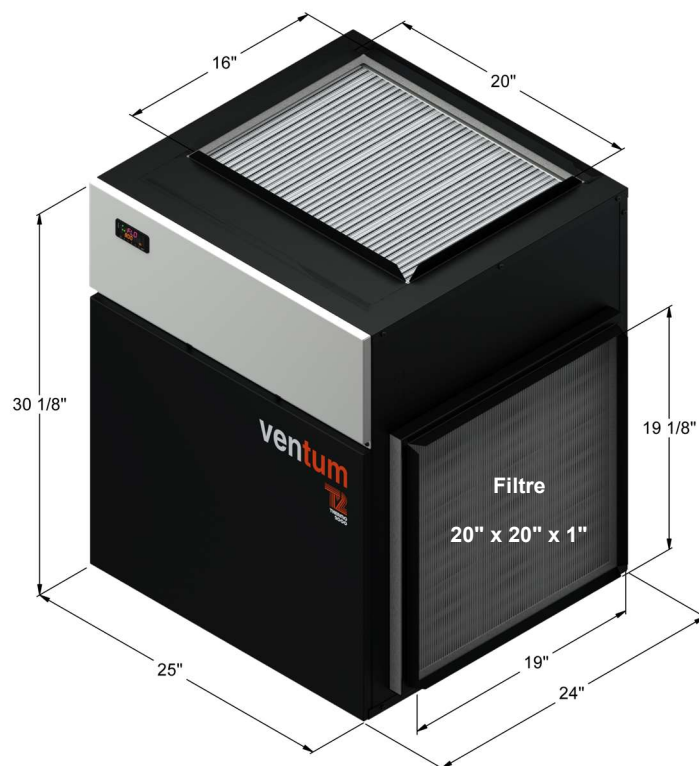
Figure 2 : Dimensions VenTum 60
